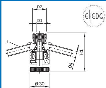
1 - optional flushing connection
