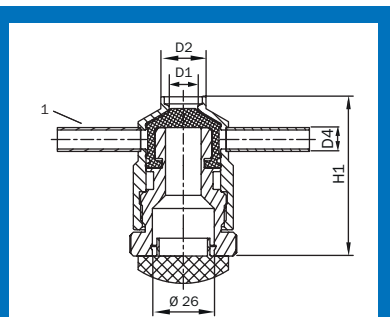
1 - optional flushing connection
